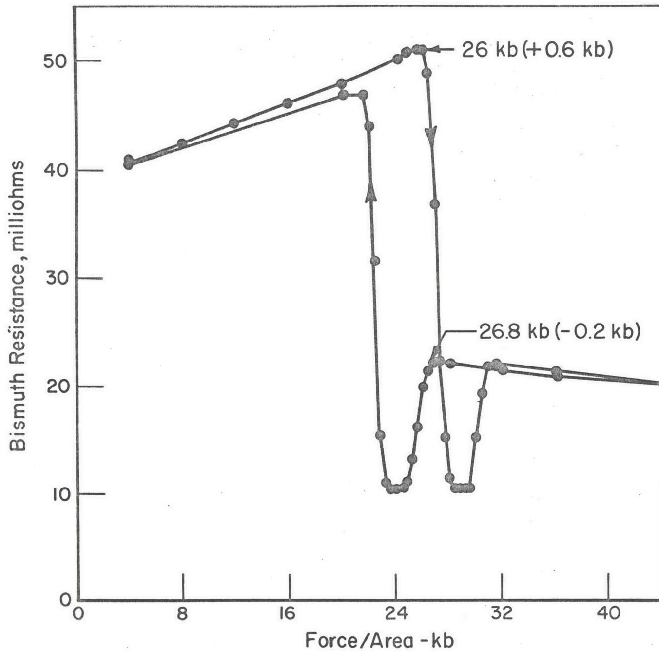
BISMUTH CALIBRATION IN AgCl PORTION OF CELL
